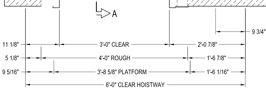
HOISTWAY PLAN
