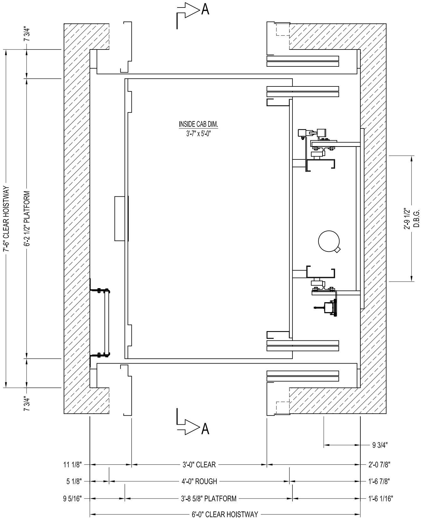
HOISTWAY PLAN
