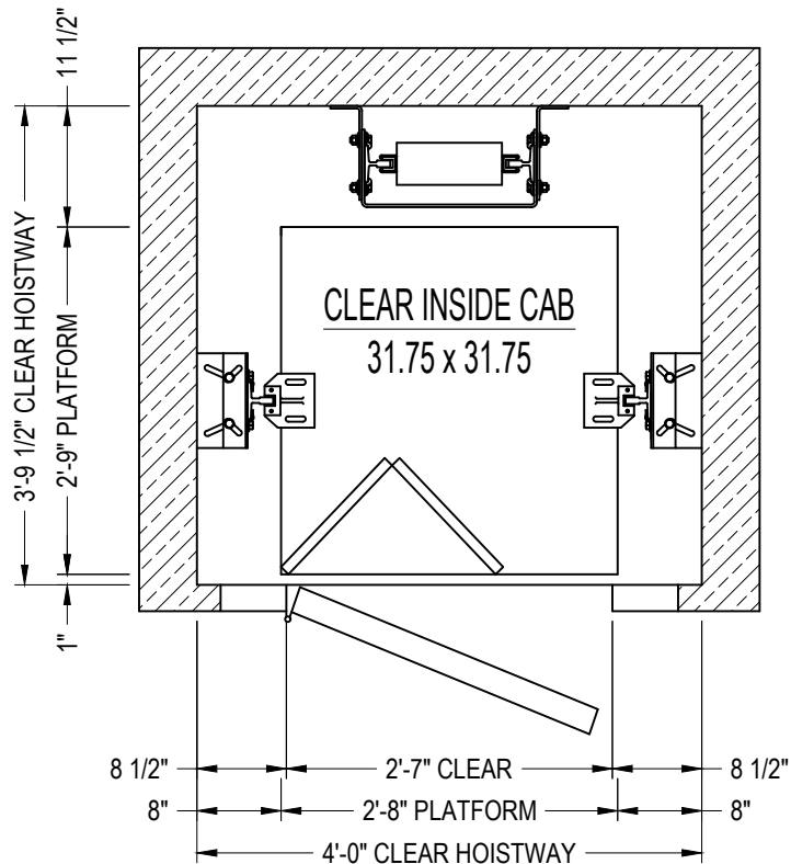
HOISTWAY PLAN
