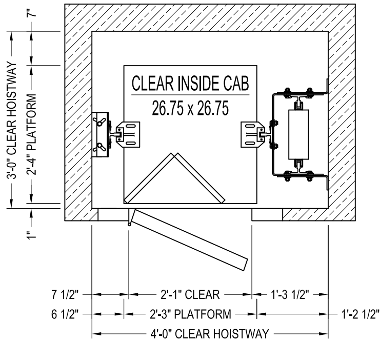
HOISTWAY PLAN
