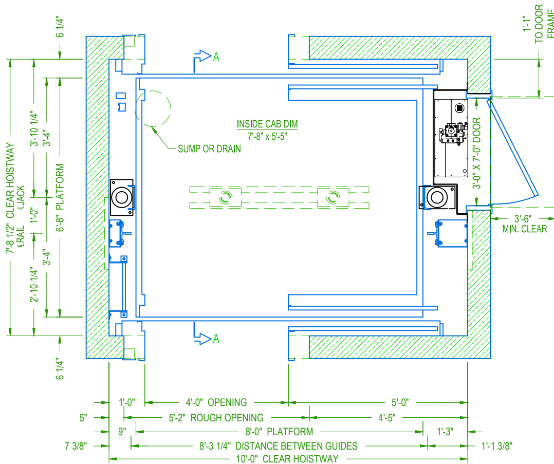
SINGLE SPEED HOISTWAY PLAN
