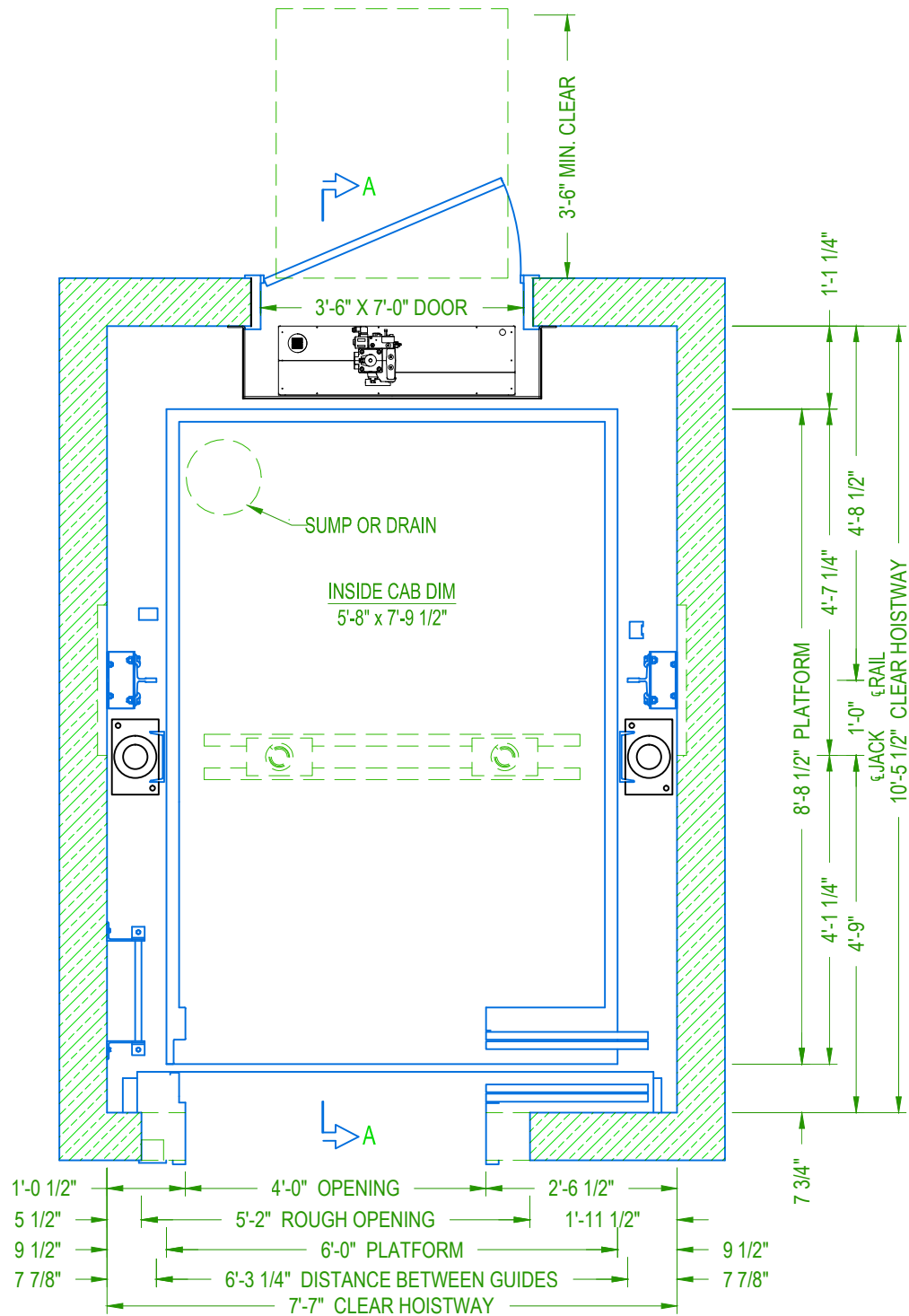
TWO SPEED HOISTWAY PLAN
