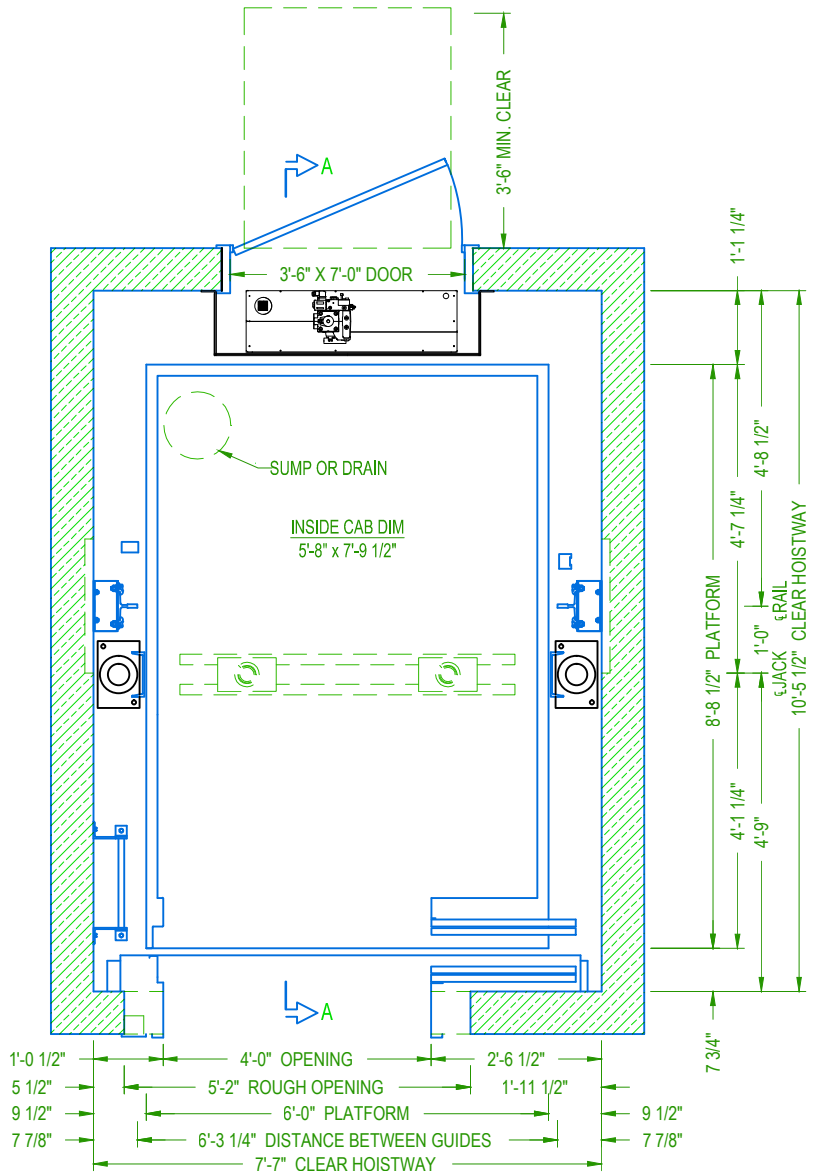
TWO SPEED HOISTWAY PLAN
