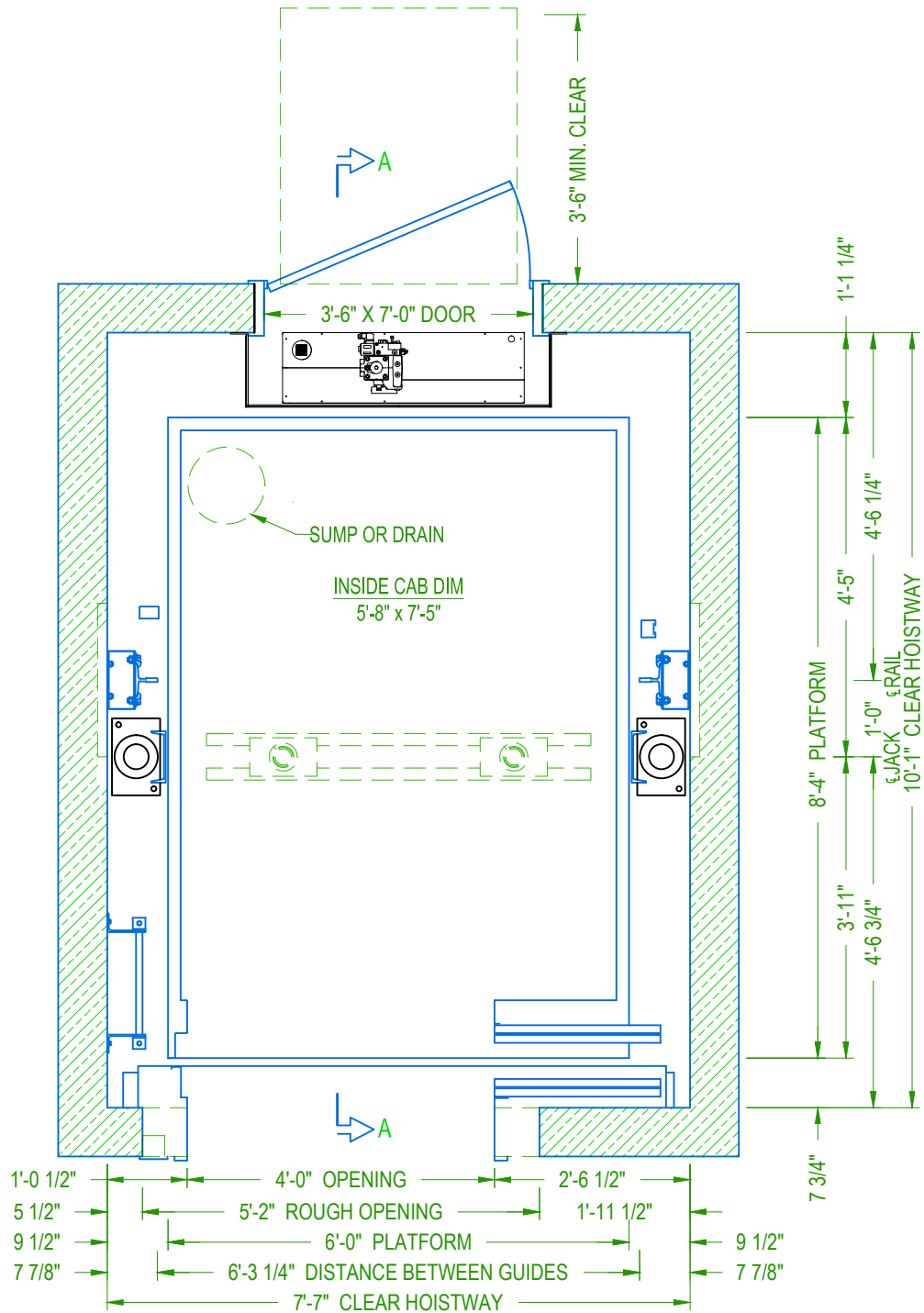
TWO SPEED HOISTWAY PLAN
