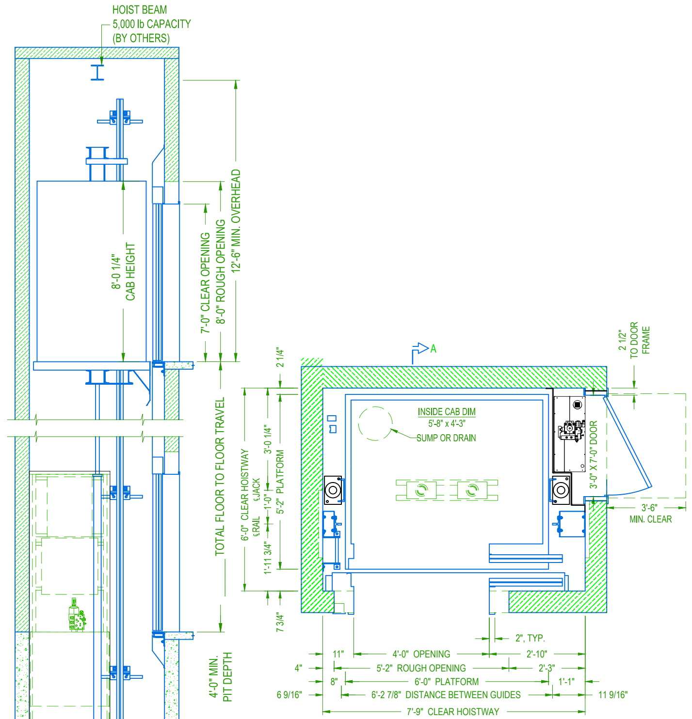
TWO SPEED HOISTWAY PLAN
