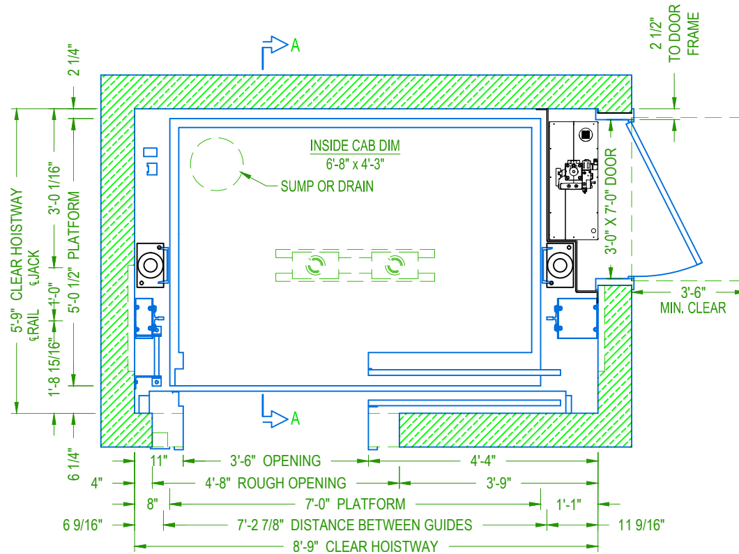
SINGLE SPEED HOISTWAY PLAN
