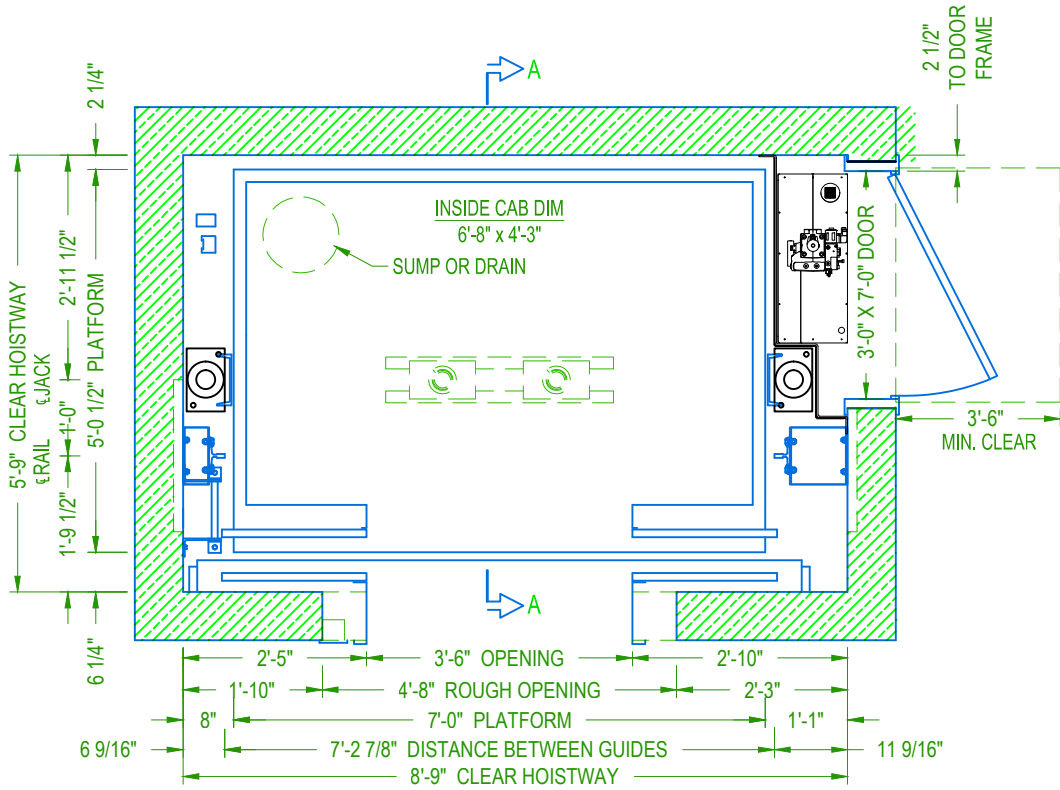
CENTER PARTING HOISTWAY PLAN
