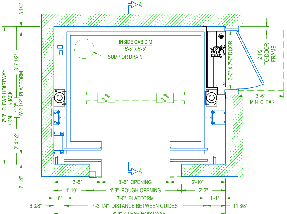
CENTER PARTING HOISTWAY PLAN
