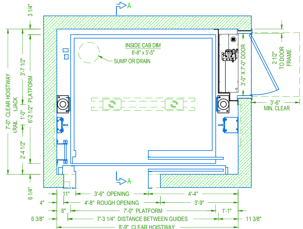
SINGLE SPEED HOISTWAY PLAN
