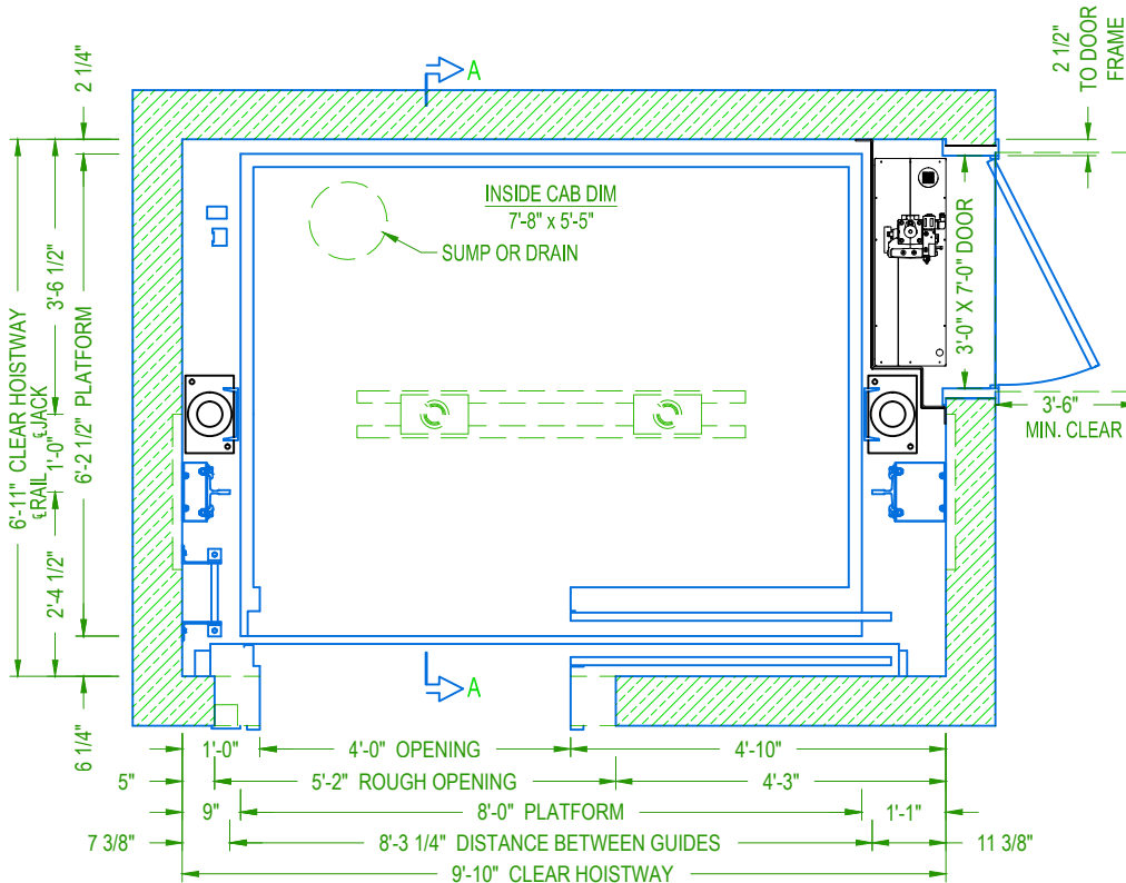
SINGLE SPEED HOISTWAY PLAN
