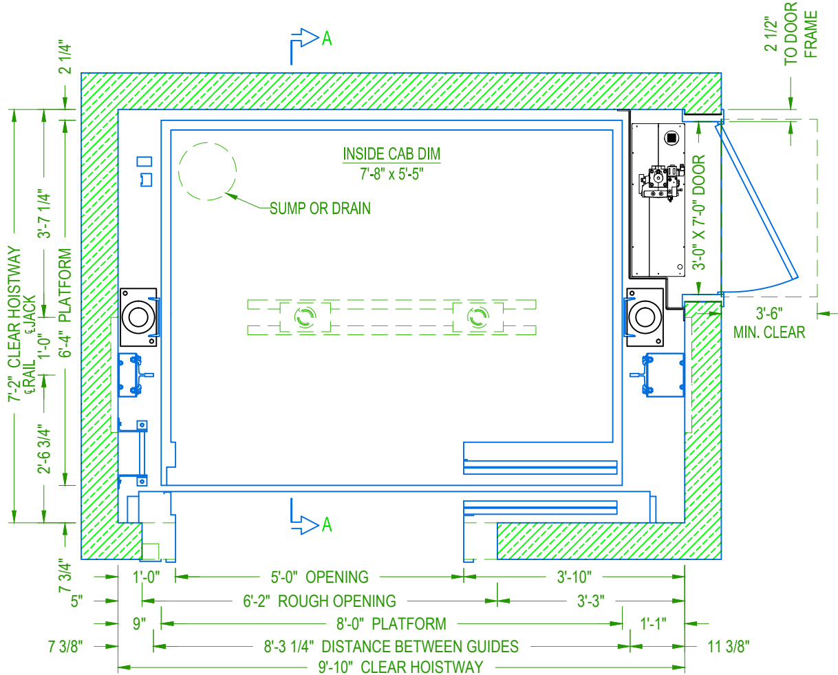
TWO SPEED HOISTWAY PLAN
