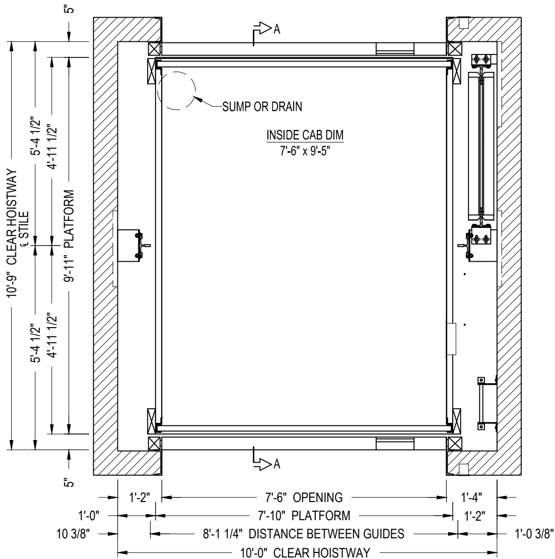
HOISTWAY PLAN
