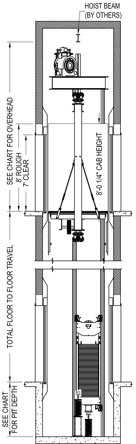
HOISTWAY ELEVATION VIEW
