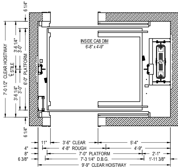
SINGLE SPEED HOISTWAY PLAN
