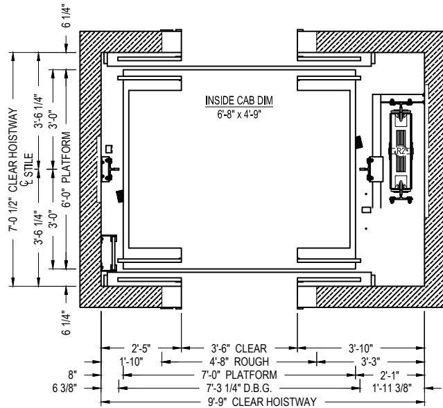
CENTER PARTING HOISTWAY PLAN
