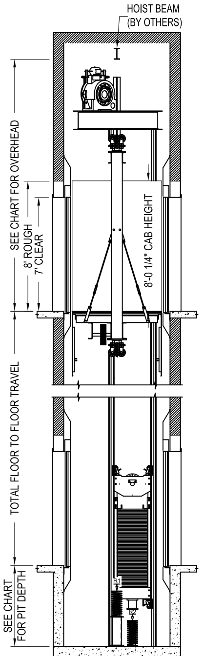
HOISTWAY ELEVATION VIEW
