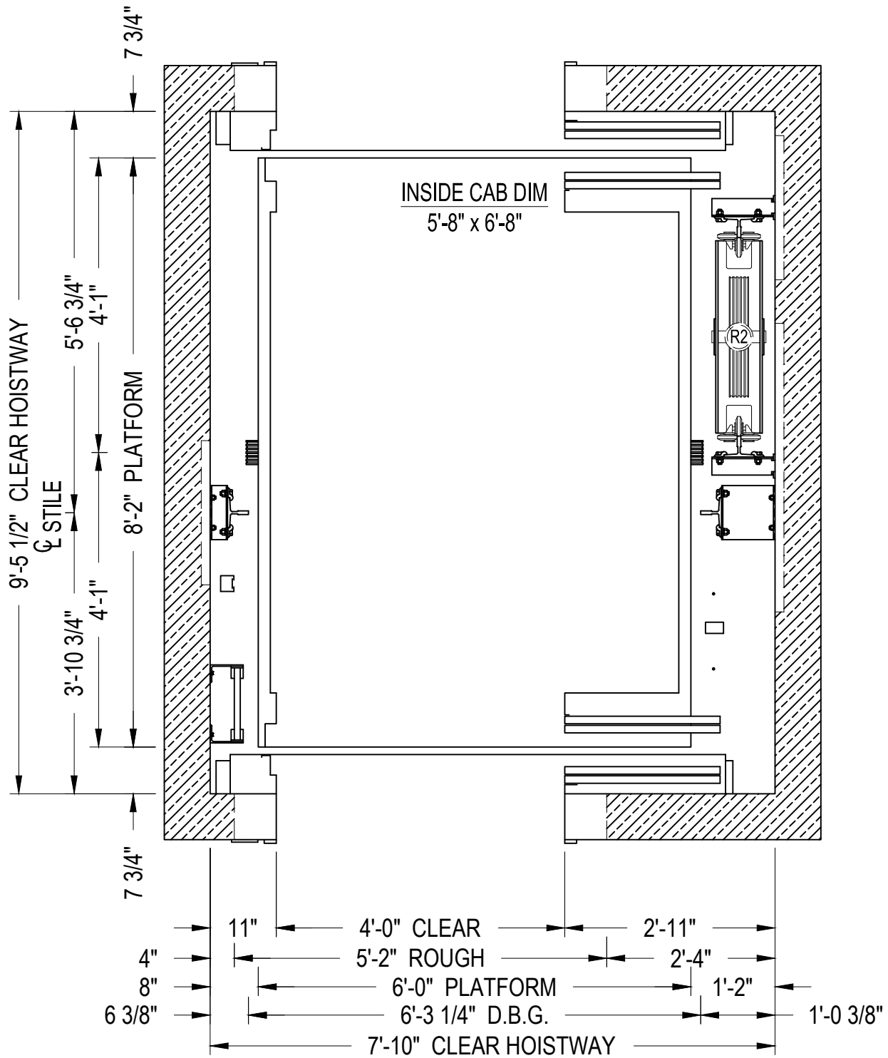
TWO SPEED HOISTWAY PLAN
