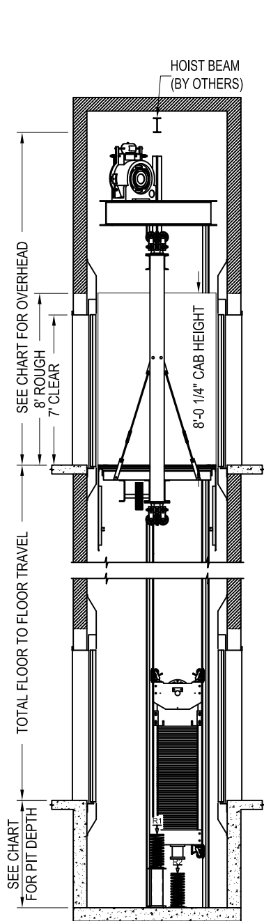
HOISTWAY ELEVATION VIEW
