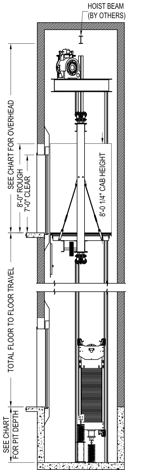
HOISTWAY ELEVATION VIEW
