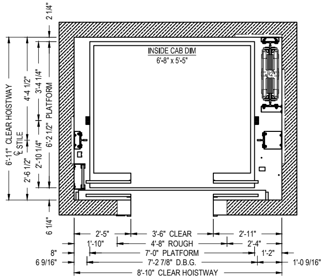
CENTER PARTING HOISTWAY PLAN
