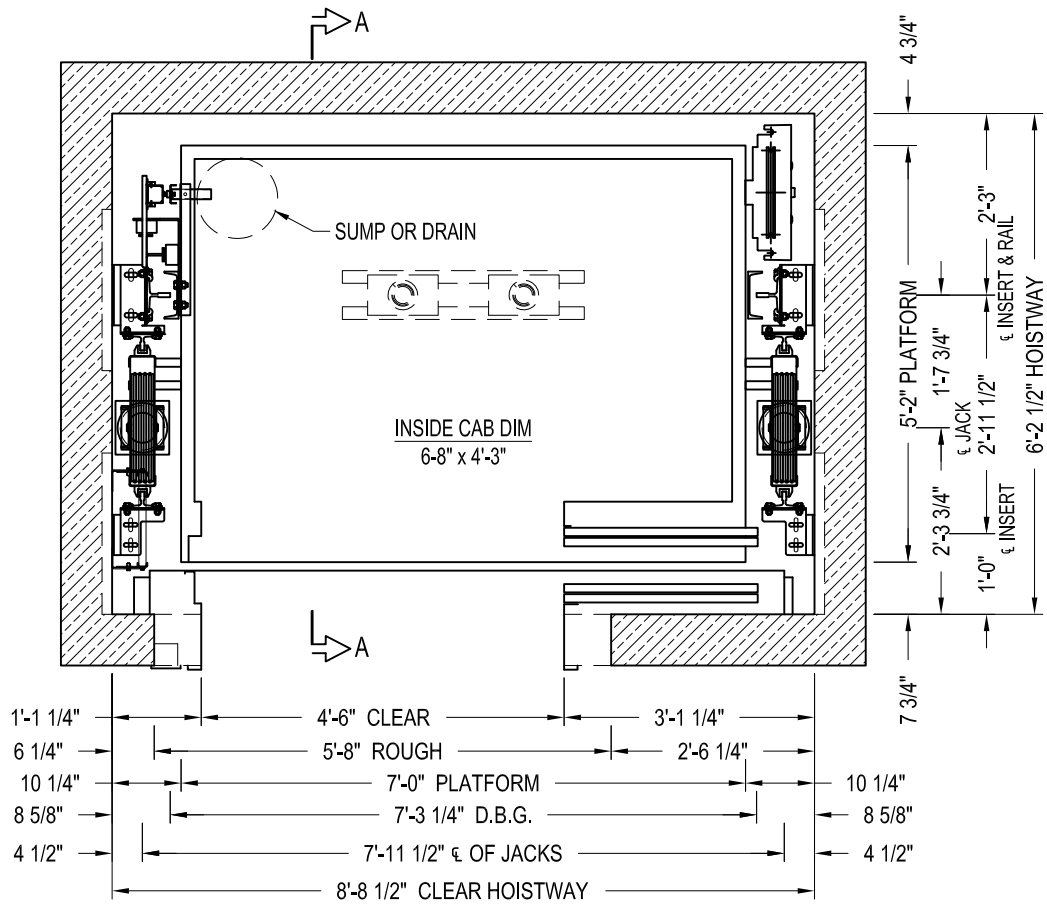
TWO SPEED HOISTWAY PLAN
