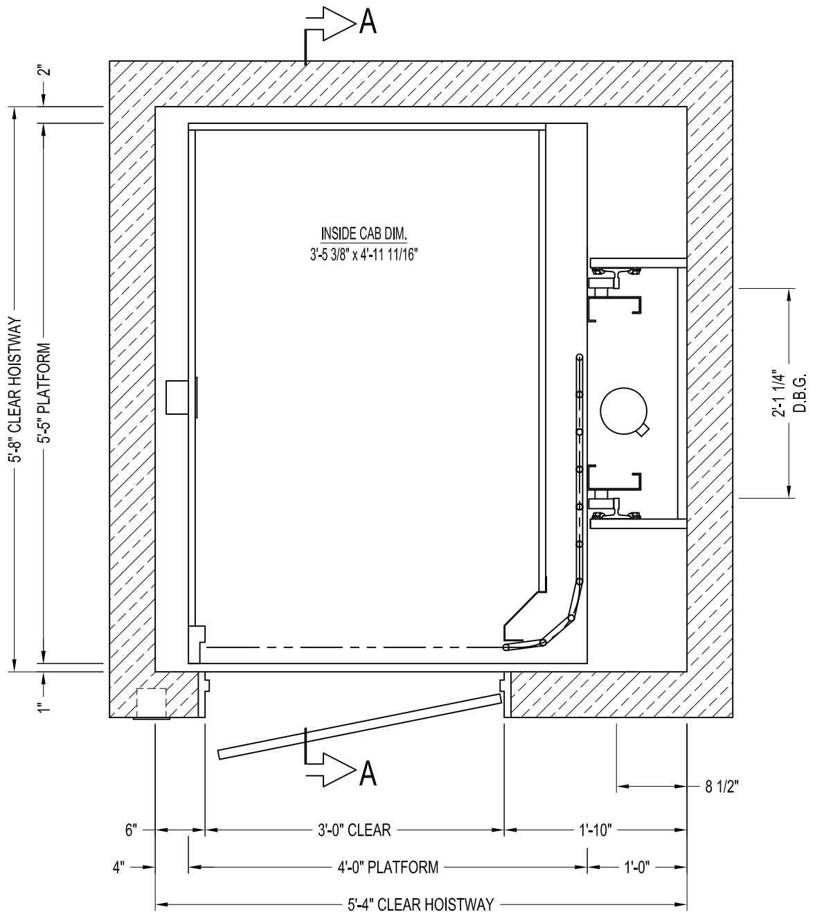
HOISTWAY PLAN
