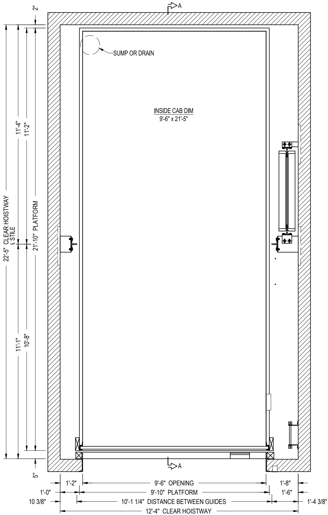
HOISTWAY PLAN
