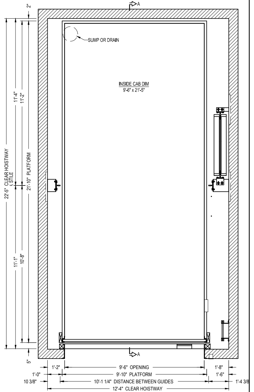
HOISTWAY PLAN
