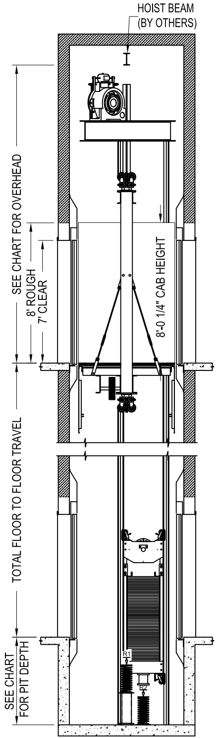
HOISTWAY ELEVATION VIEW
