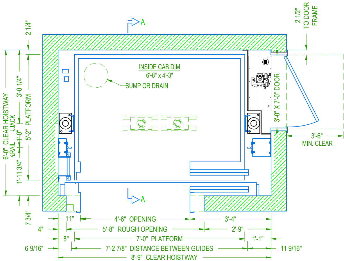
TWO SPEED HOISTWAY PLAN
