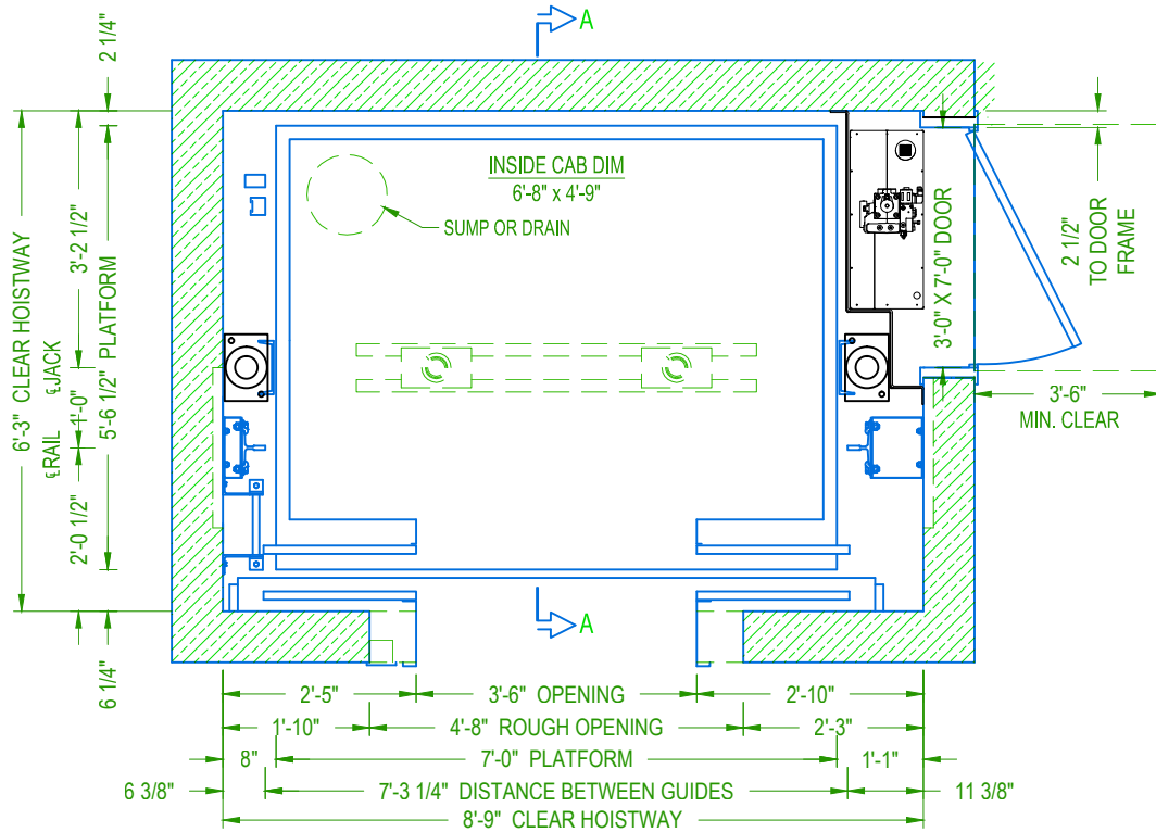
CENTER PARTING HOISTWAY PLAN
