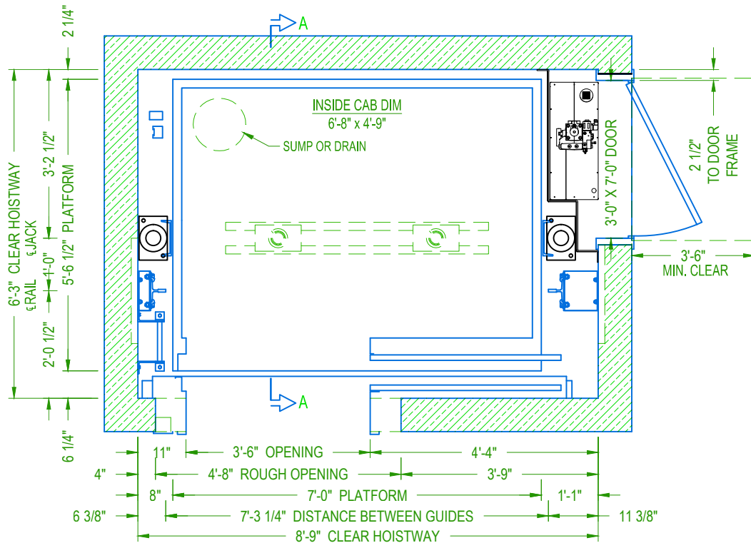
SINGLE SPEED HOISTWAY PLAN
