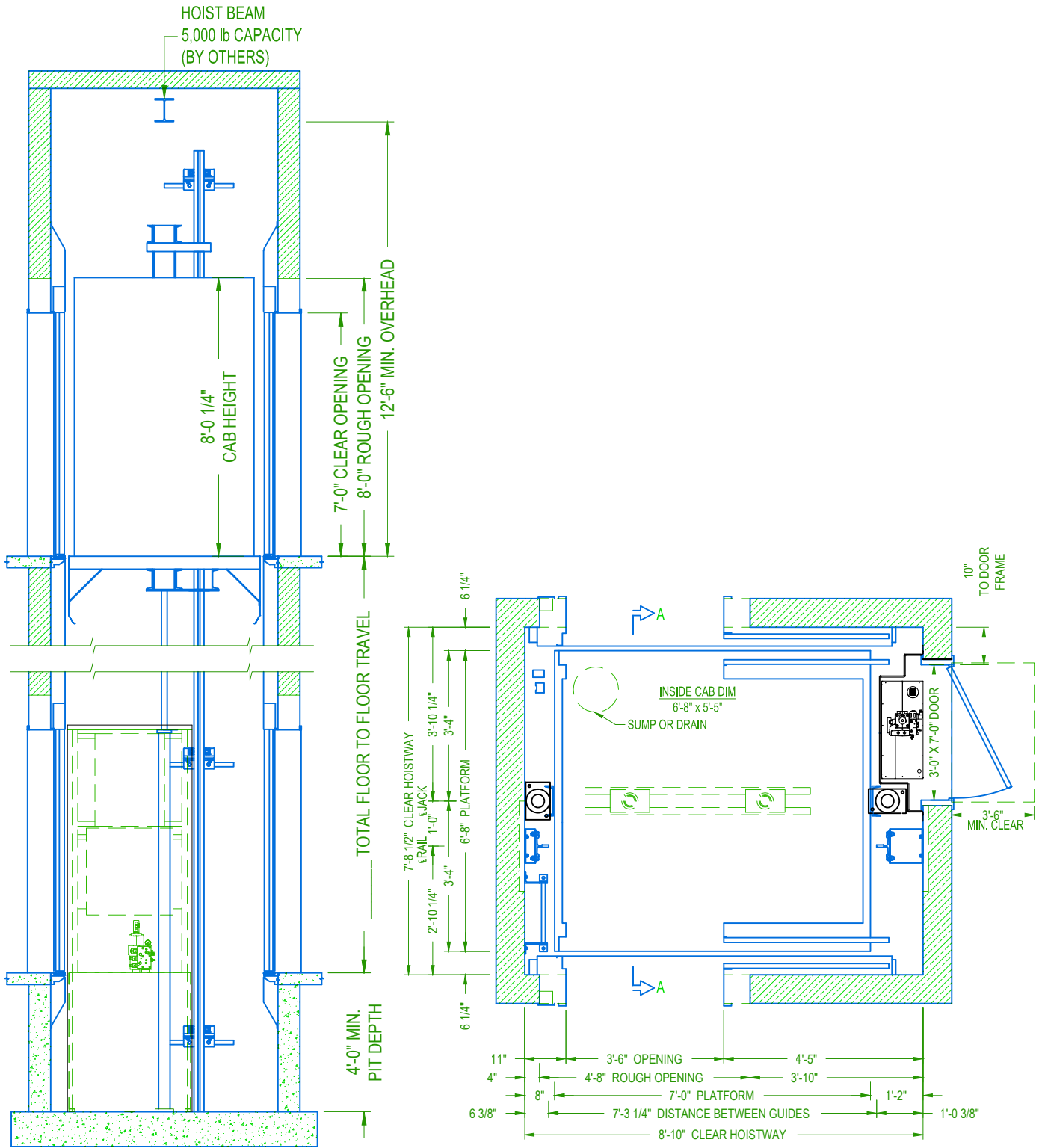
SINGLE SPEED HOISTWAY PLAN
