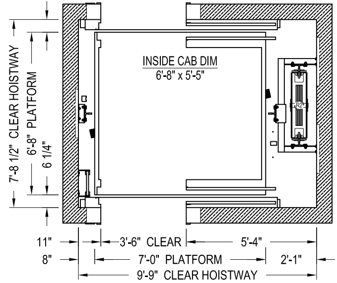
SINGLE SPEED HOISTWAY PLAN
