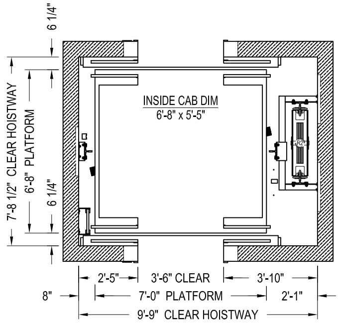
CENTER PARTING HOISTWAY PLAN
