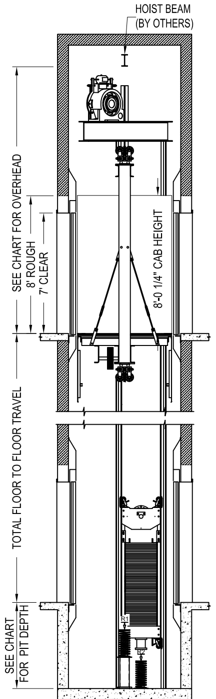
HOISTWAY ELEVATION VIEW
