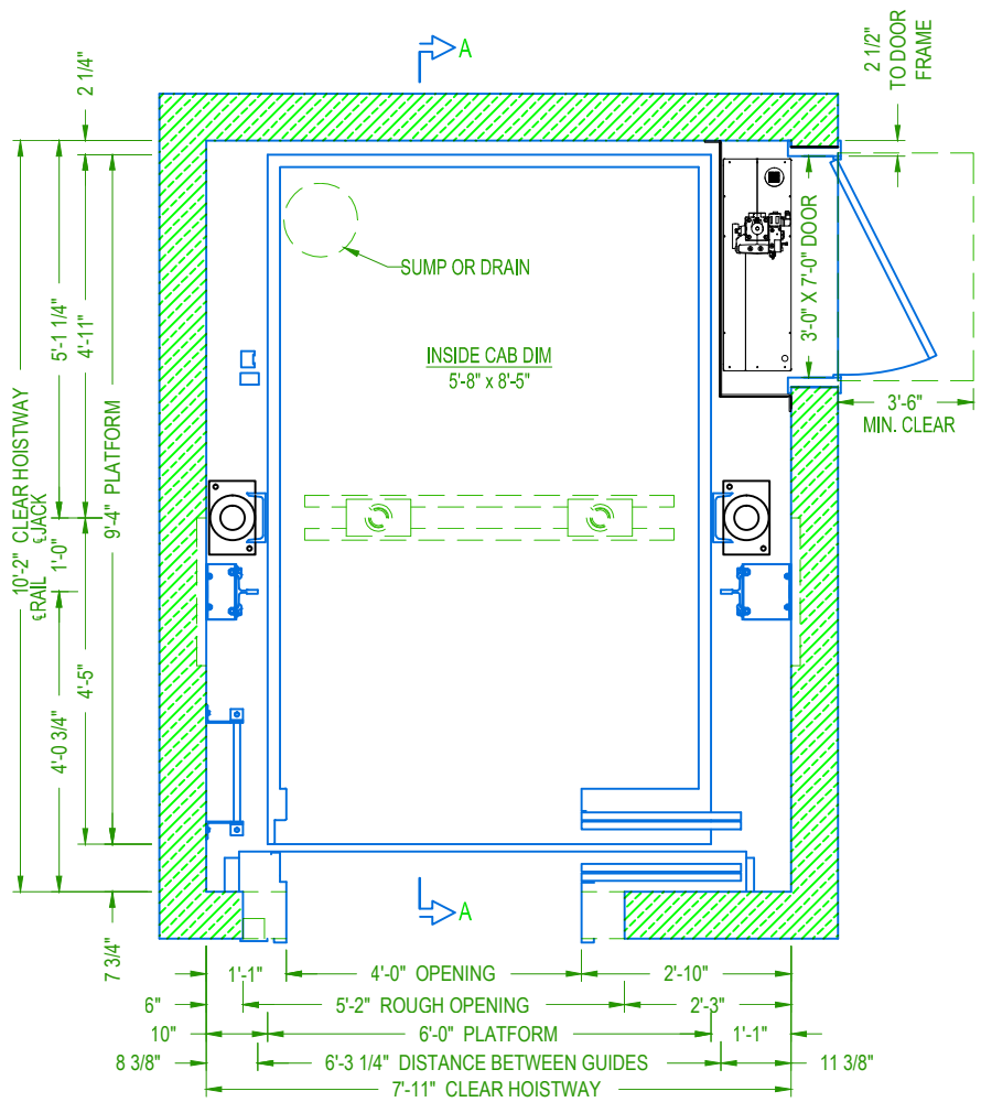
TWO SPEED HOISTWAY PLAN
