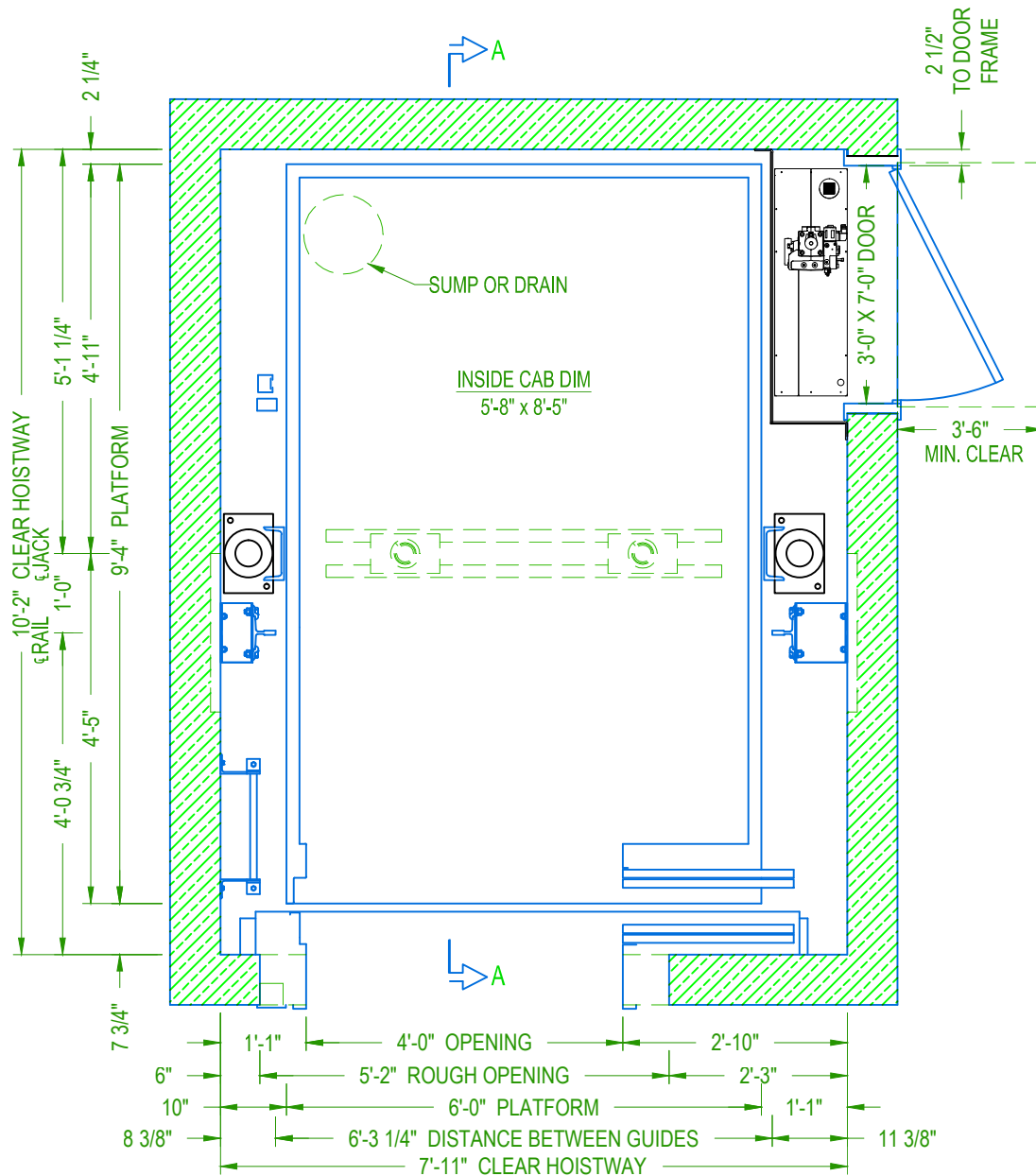
TWO SPEED HOISTWAY PLAN
