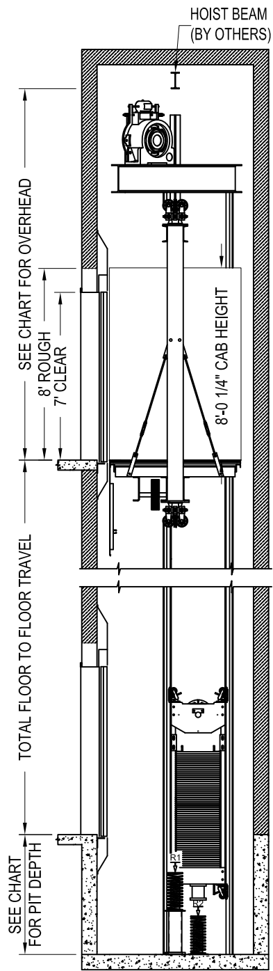
HOISTWAY ELEVATION VIEW
