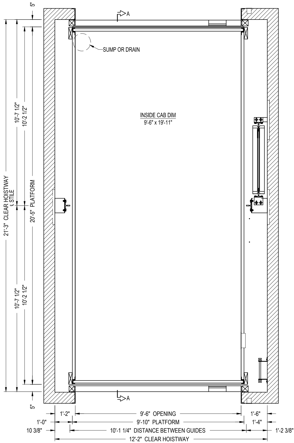
HOISTWAY PLAN
