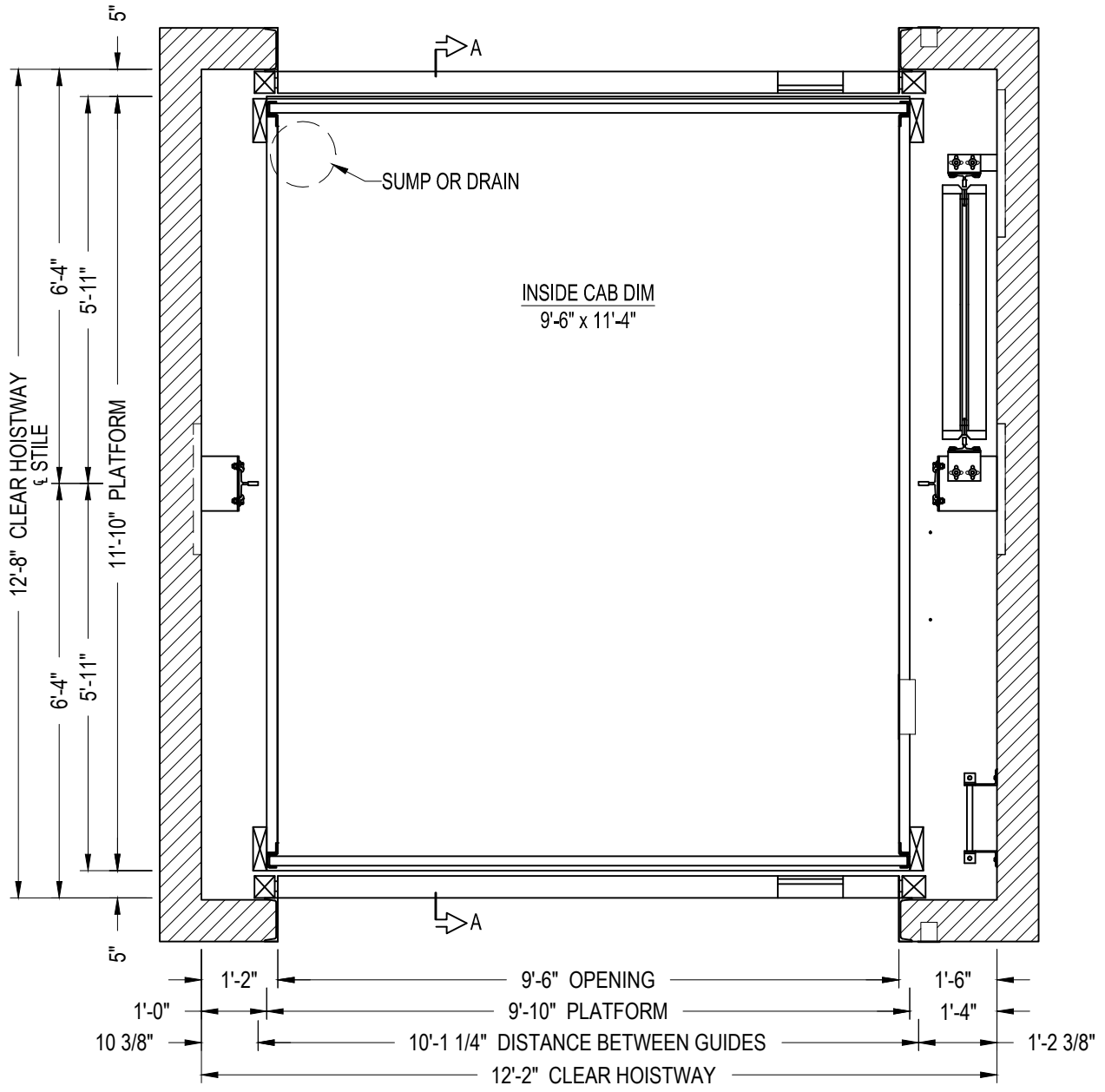
HOISTWAY PLAN
